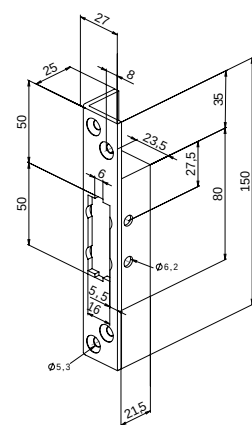
Angled striking plate
