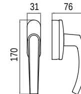
YBZW04 L/R Outward-open fork handle
