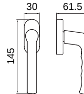
YFZ01 Inward-open spindle handle
