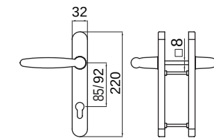
YMSZ9205 / YMSZ8505 Integrated Door handle
