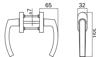
YSMZ06 Separated Door handle
