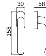
YFZ04 Inward-open spindle handle
