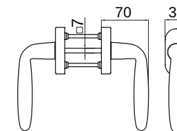
YSMZ07 Separated Door handle
