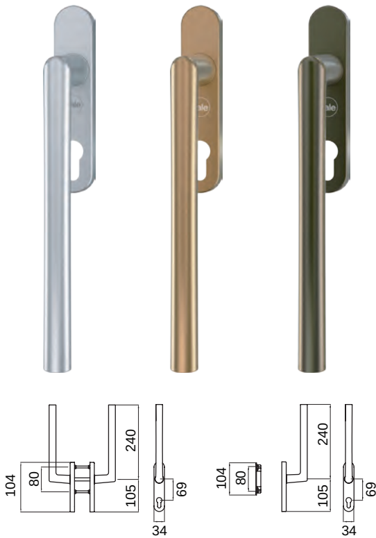
YTMSZ6901100 | YTMSZ6902060 Lifting & sliding door handle
