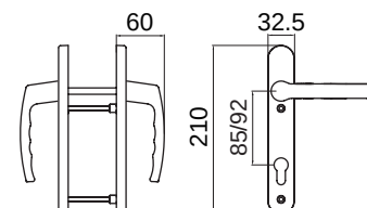
YMSZ9202 | YMSZ8502 Integrated Door handle
