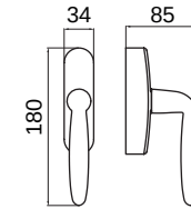
YBZ0825 T&T open handle
