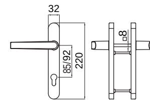
YMSZ9204 / YMSZ8504 Integrated Door handle
