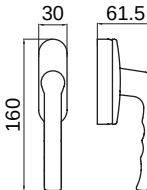
YBZW02 L/R Outward-open fork handle
