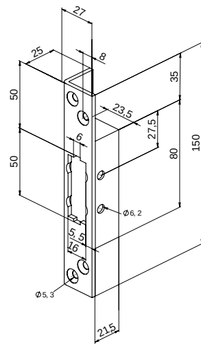
Angled striking plate
