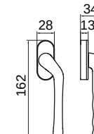
YFZS01 L/R Inward-open for spindle handle
