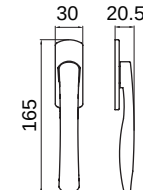
YFZ302 Inward-open for spindle handle
