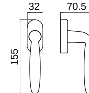
YFZ07 Inward-open spindle handle
