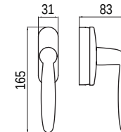
YBZW05 L/R Outward-open fork handle
