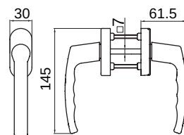
YSMZ04 Separated Door handle
