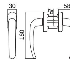
YSMZ02 Separated Door handle
