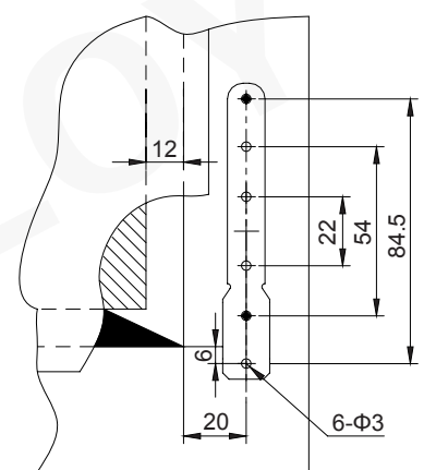
Installation Dimension of Bottom Hinge
