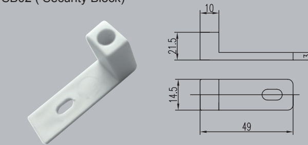
SB02 ( Security Block)
