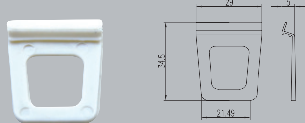
WH29 (Screen Window Handle)
