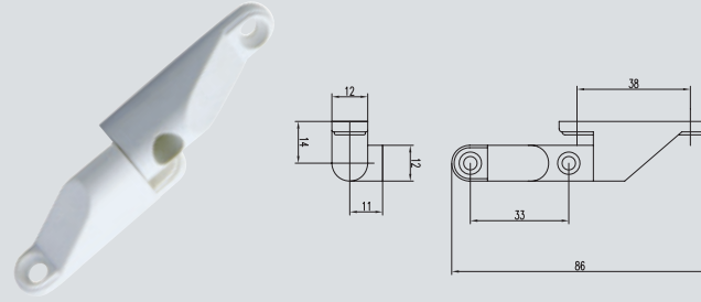
2520(Screen Window Hinge) material: zink alloy WH86(Screen Window Hinge) material: Nylon
