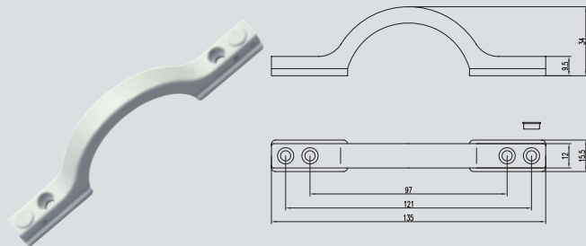
WH135 (Screen Window Handle)
