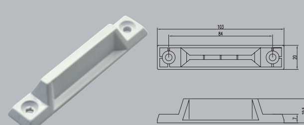
WH127 (Screen Window Handle)
