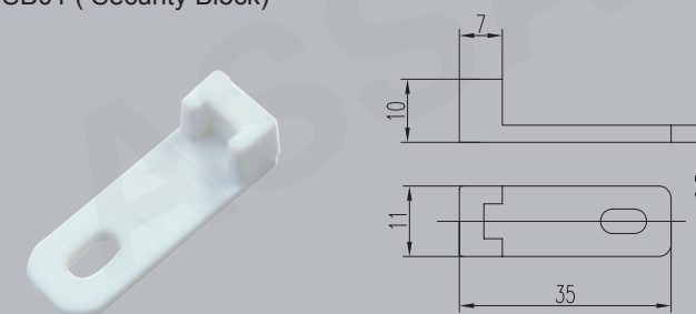
SB01 ( Security Block)
