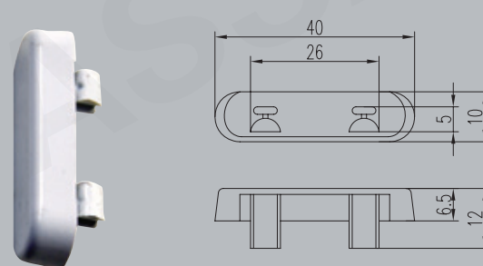
HC 11 (Drain Hole Cover)
