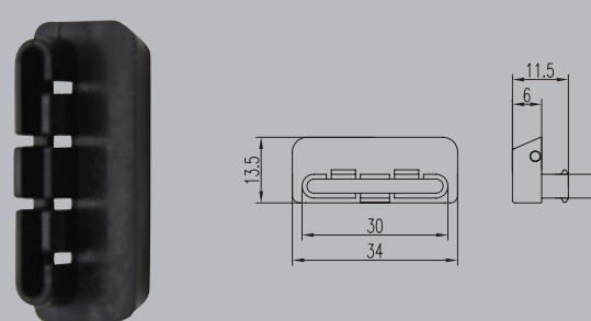
HC 12 (Drain Hole Cover)
